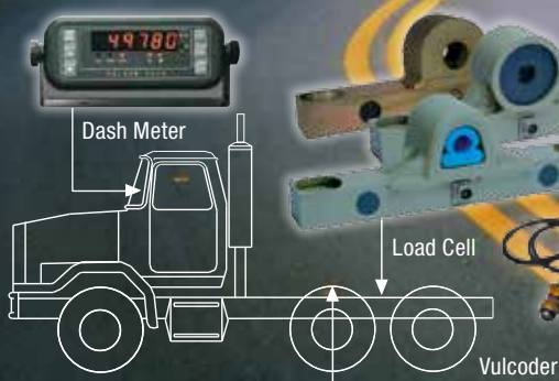
Fifth Wheel
