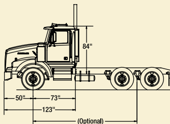
4900 SA (Set-back, Super Visibility Hood) 109" and 123" BBC; 50" BA
