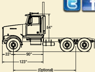
4900 FA (Set-forward) 109" and 123" BBC; 33" BA
